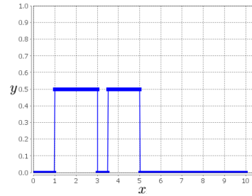
Fig. 2: FSs generated from the intervals \bar{A}_1 = [2, 4] and \bar{A}_2 = [2, 4] for Fig. (2a), and the intervals \bar{A}_1 = [1, 3] and \bar{A}_2 = [3.5, 5] for Fig. (2b).
