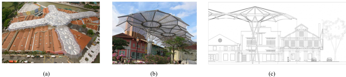
Fig.5. (a & b) Aerial and street view of the ETFE structure at Clark Quay; (c) Clarke Quay ETFE structure at 15m above ground (source: Archinnet)
