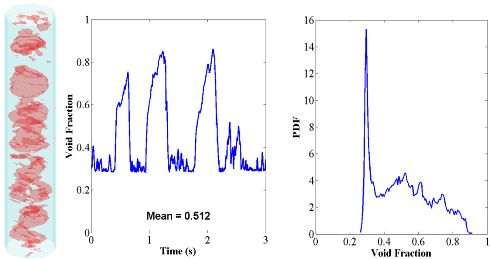
Slug flow; valve setting = 1.0
