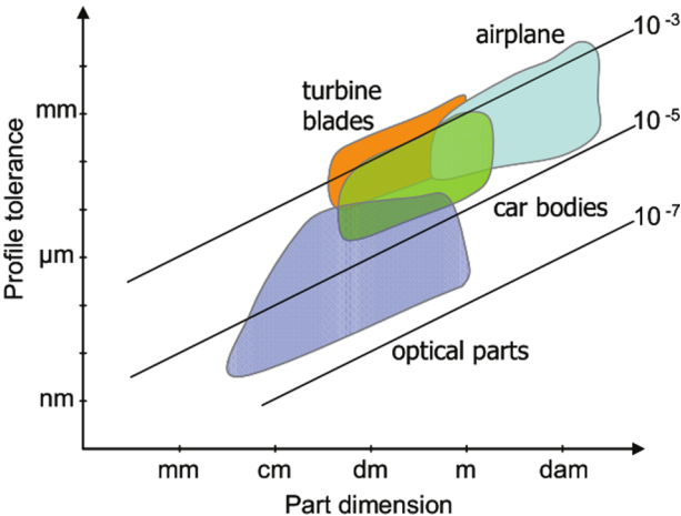
FIG. 2. Tolerance against part dimension for various industrial applications. 16 Reprinted with permission from E. Savio, L. De Chiffre, and R. Schmitt, CIRP Ann.–Manuf. Technol. 56 , 810–835 (2007). Copyright 2007 Elsevier.
