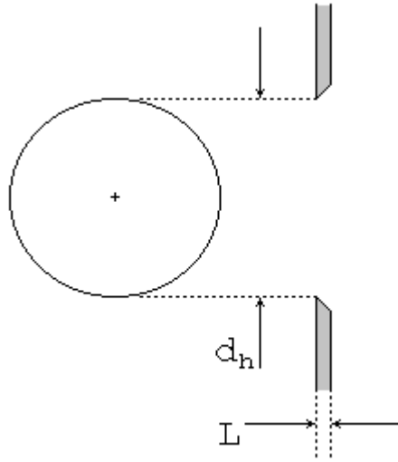
Figure 1: Circular sharp-edged orifice where d_h \gg L .
