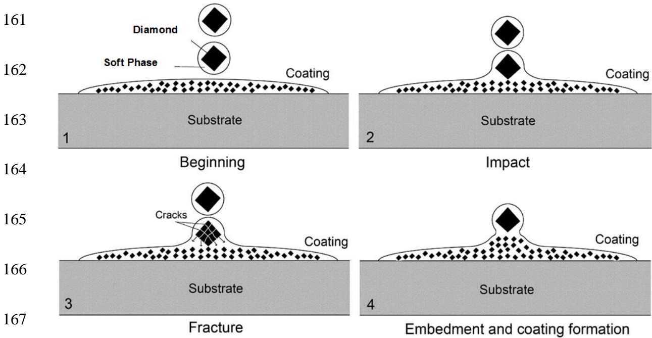
Fig. 4 Metal-coated Diamond composite coating formation mechanism
