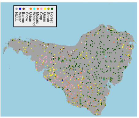
Fuzzy Sets
