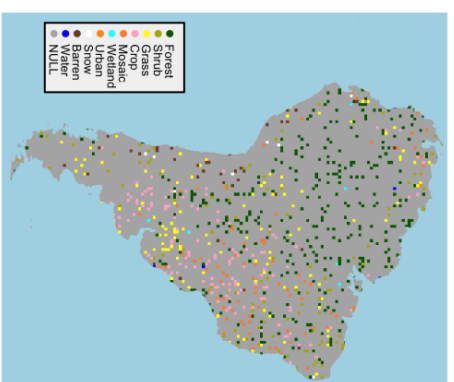
Bayesian Prob
