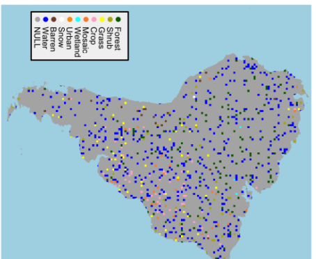
Dempster-Shafer
