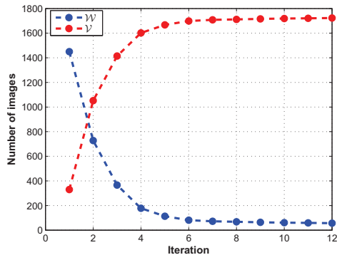
Figure 4: The cardinality of \mathcal{W} and \mathcal{V} per iteration.
