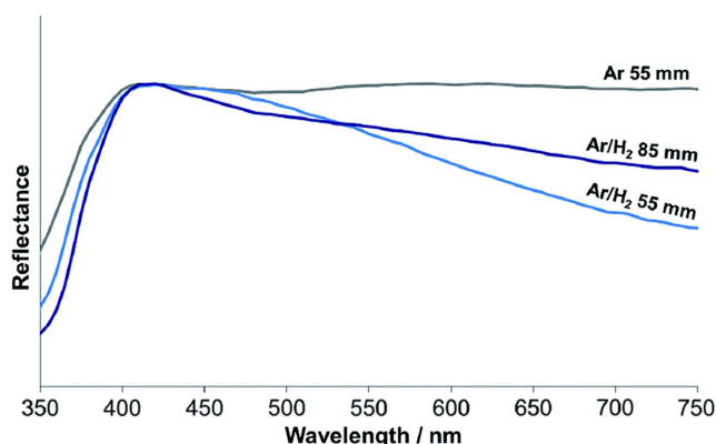
Figure 18. UV-vis reflectance spectra of TiO 2 coatings produced in the two plasma conditions. Reproduced with permission. [106] Copyright Royal Society of Chemistry.
