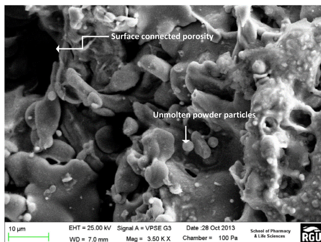
Figure 5. Scanning electron microscope (SEM) images of APS-coated anode layer surfaces showing surface-connected porosities and unmolten powder particles (Mo–Mo 2 C/ZrO 2 ). Reproduced with permission. [31] Copyright 2015, Springer Nature.
