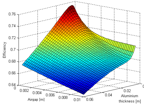
Figure 3 Airgap and aluminum thickness effect on the efficiency
