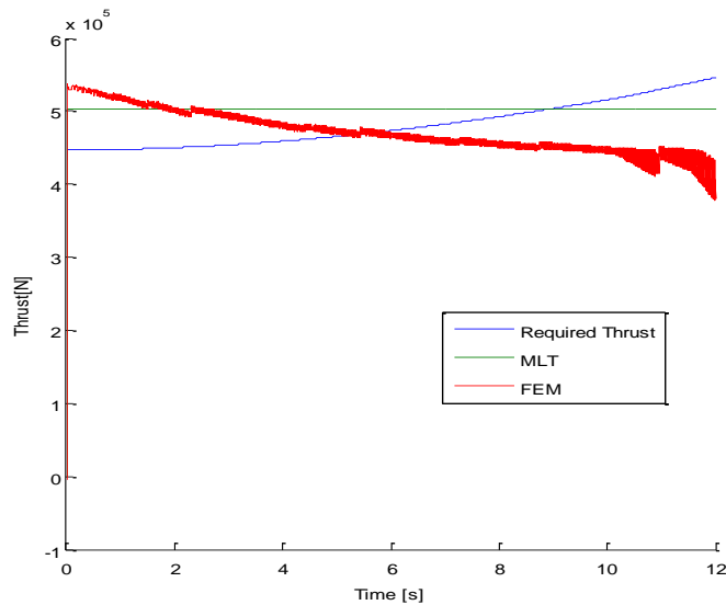
Figure 8: MLT and FEA results comparison
