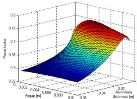
Figure 4 Airgap and aluminum effect on power factor
