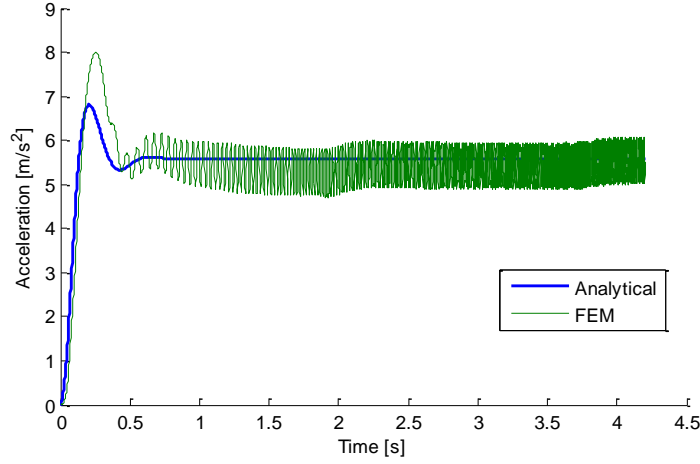
Figure 6: Circuit model and FEA results comparison
