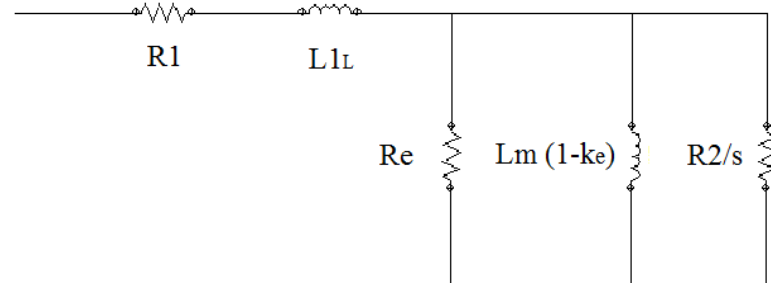
Figure 5: LIM equivalent circuit
