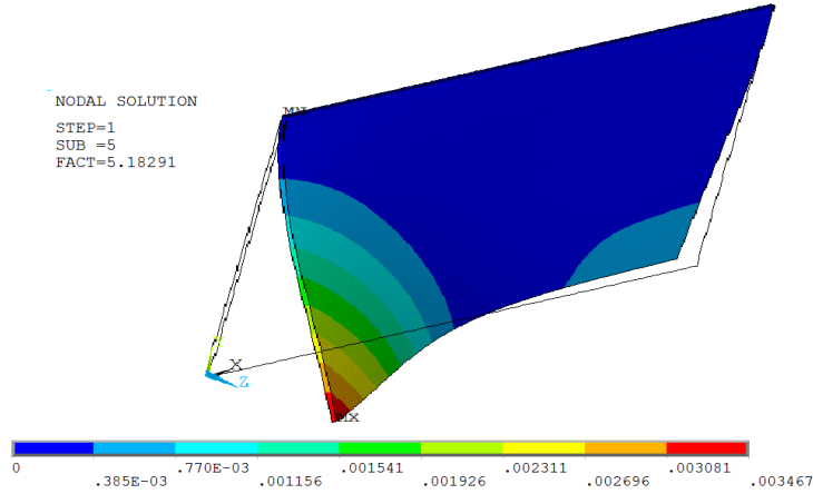
Figure 9: Exaggerated plate deformation under buckling load
