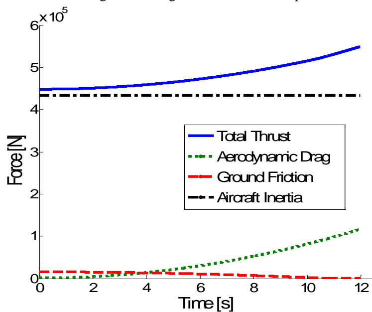
Figure 2: Forces acting on A320 during take-off at 0.6G constant acceleration
