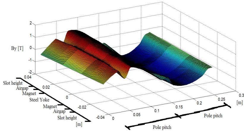
Figure 7: Field density generated by a pole pair with slotting effect
