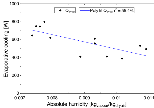
Figure 7 IDCS evaporative-inter cooler output with inlet air absolute humidity
