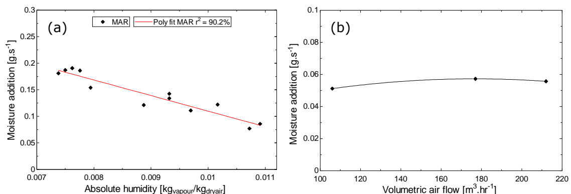
Figure 9 IDCS regenerator performance with (a) inlet air absolute humidity, and (b) volumetric air flow
