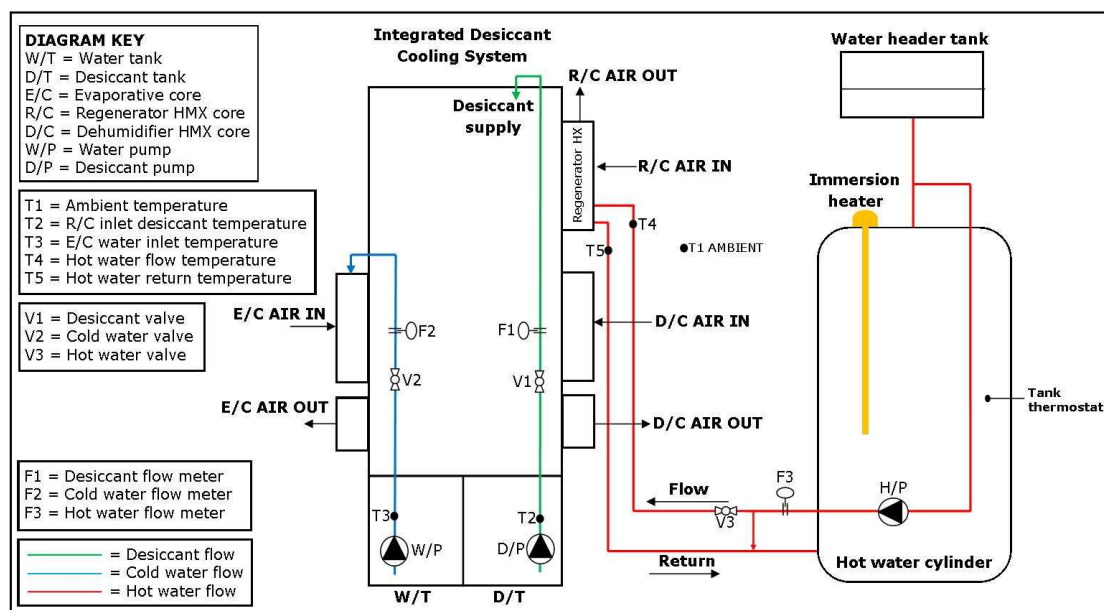
Figure 2 System schematic of the IDCS laboratory set-up
