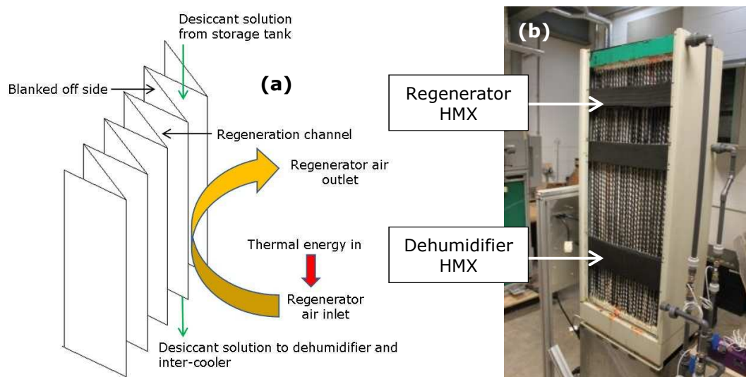
Figure 3 (a) Regenerator core operating concept, and (b) the regenerator HMX
