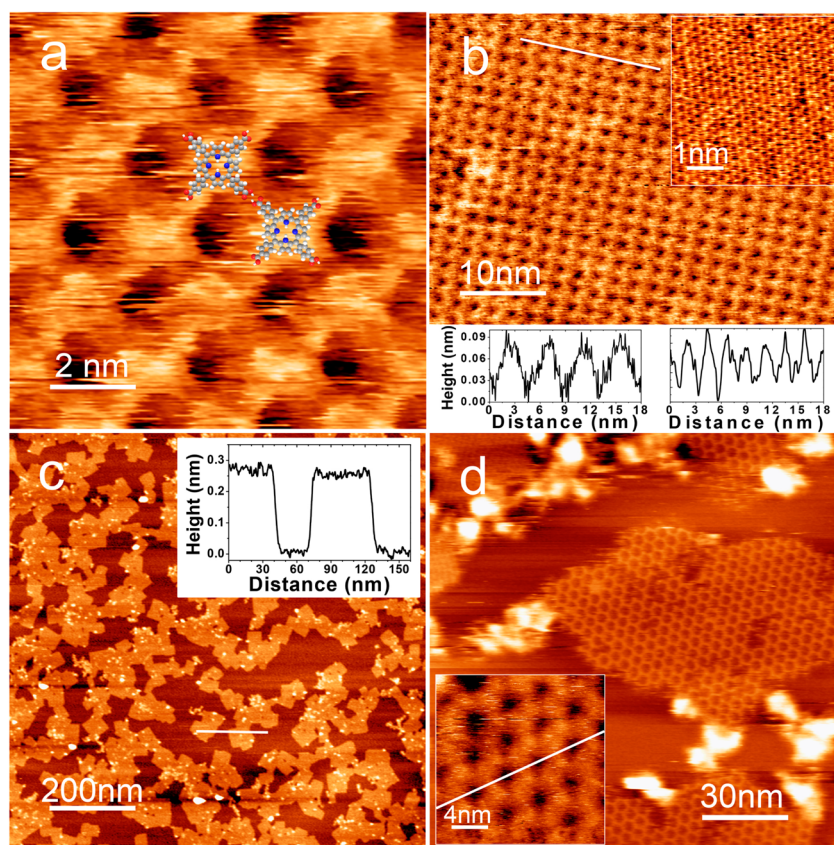
Figure 1. AFM images of TCPP adsorbed on hBN by immersion for 10 s in a 13 \mu\text{M} EtOH solution. (a) High-resolution scan of square TCPP phase; (b) larger area image showing square phase (upper inset) hBN lattice and (lower inset) height profiles of square and hexagonal arrays extracted from images along highlighted white lines in b (right) and d (left); (c) overview image of island morphology of TCPP; (d) hexagonal phase of TCPP; inset presents zoom-in showing additional detail and placement of the line along which profile in b is extracted. Images were acquired in (a) contact mode and (b–d) ac mode using an Asylum Cypher AFM.
