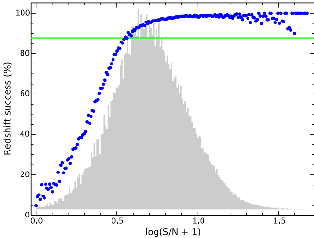
Figure 10. The blue points show redshift success, i.e. the fraction of spectra of main survey targets with secure redshifts, as a function of the spectral S/N per pixel, averaged over the full spectrum (excluding bad pixels). The horizontal green line shows the survey’s overall redshift success, while the grey shaded histogram shows the S/N distribution of the spectra (on an arbitrary linear scale).
