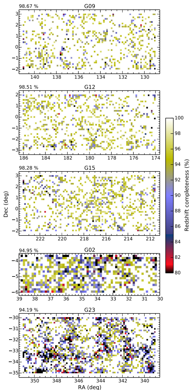
Figure 16. Redshift completeness of the five GAMA II survey regions, as indicated, in bins of 0.14^\circ size. For G02, we only show the high-priority subregion. The average completeness of each region is indicated at the top left of each panel.
