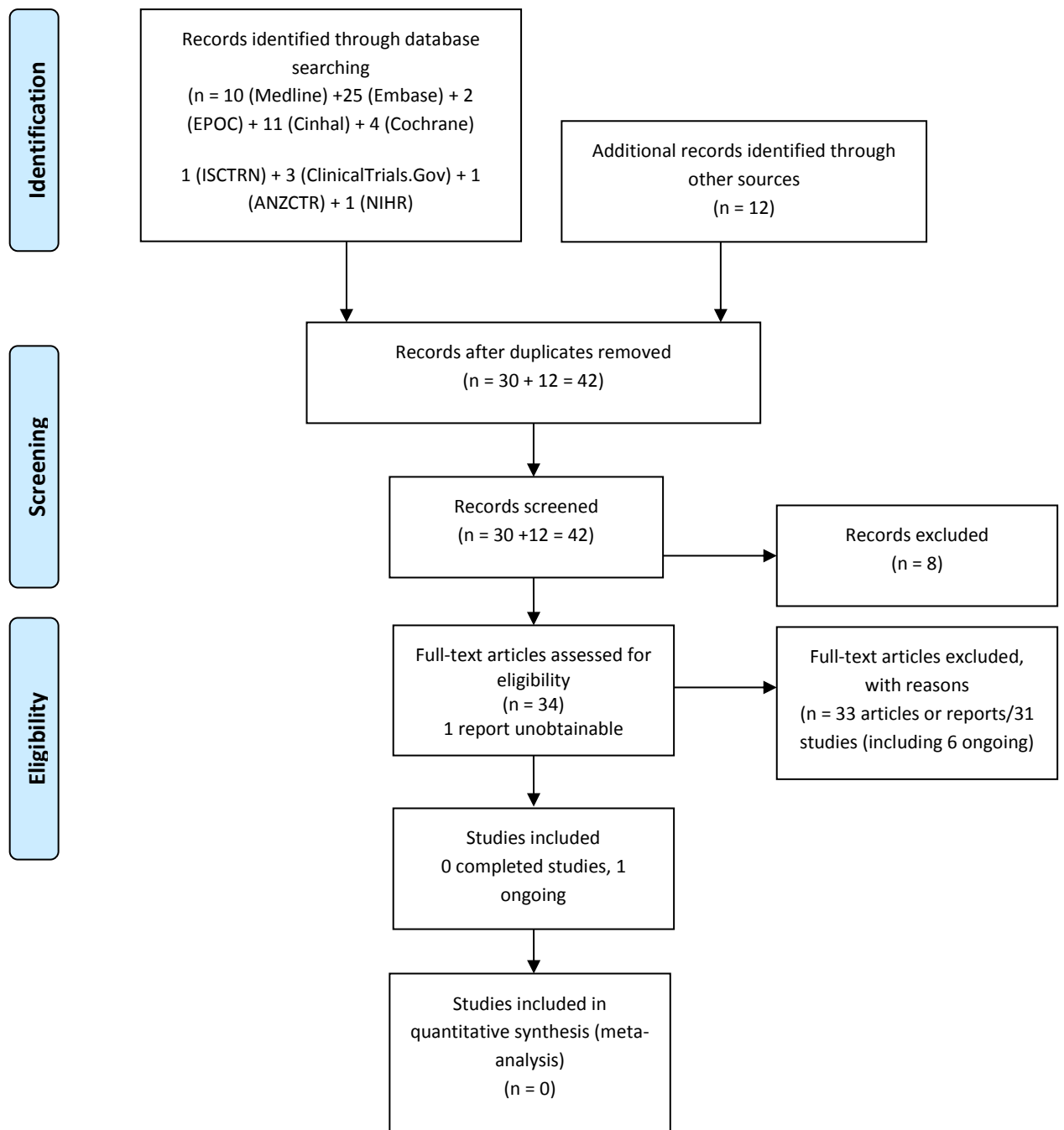
Diagram 1 PRISMA flowchart
