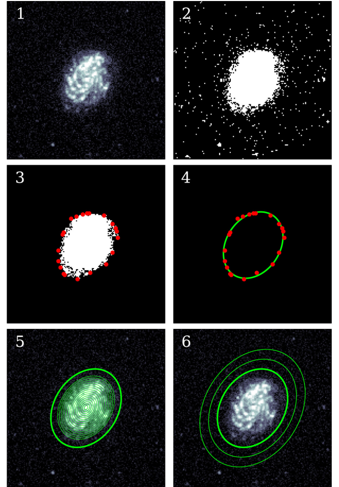
Figure 4. Illustration of the stages of our aperture-fitting process, using GALEX FUV imagery of galaxy NGC 5584 (HAPLESS 14) as an example. Panel 1 shows the inner 500 arcsec \times 500 arcsec portion of the cutout centred upon the target source. Panel 2 shows all of the pixels in the cutout with SNR > 3 . Panel 3 shows the significant pixels of the target source, contained within their convex hull (red points). Panel 4 shows an ellipse fitted to the convex hull; this ellipse provides the position angle and axial ratio of the source aperture. Panel 5 depicts the incremental annuli used to establish the semimajor axis at which annular flux falls to SNR < 2 (thin concentric lines); 1.2 times this distance is then used as the semimajor axis of the source aperture (thick line). Panel 6 demonstrates the final source aperture (thick line) and sky annulus (thin lines). The apertures at all bands for a given source are then compared to select the largest, which is then employed for all bands.
