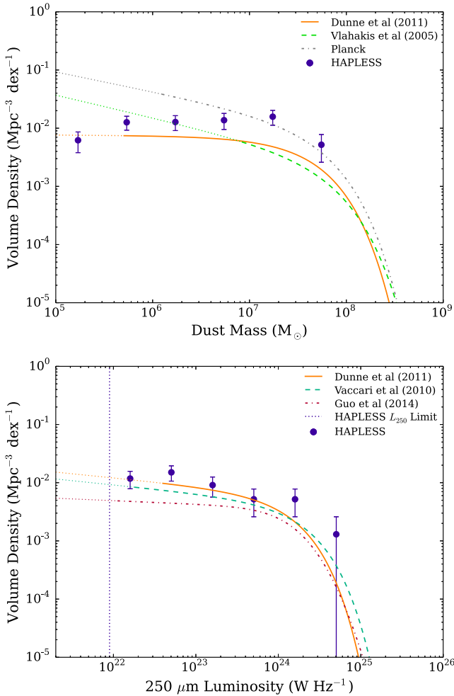
Figure 10. Upper: the HAPLESS DMF (with appropriate incompleteness corrections applied) compared with those of Planck C13N13, Vlahakis et al. (2005), and the H-ATLAS SDP functions from Dunne et al. (2011). Lower: the 250 \mu\text{m} luminosity function of HAPLESS compared with the z < 0.1 H-ATLAS samples from Dunne et al. (2011), Guo et al. (2014) and the z < 0.2 sample from HerMES (Vaccari et al. 2010). The error bars on points represent Poisson uncertainty. The functions are plotted as dotted lines in the regions where they are extrapolated. All have been adjusted to our \kappa_d and cosmology.
