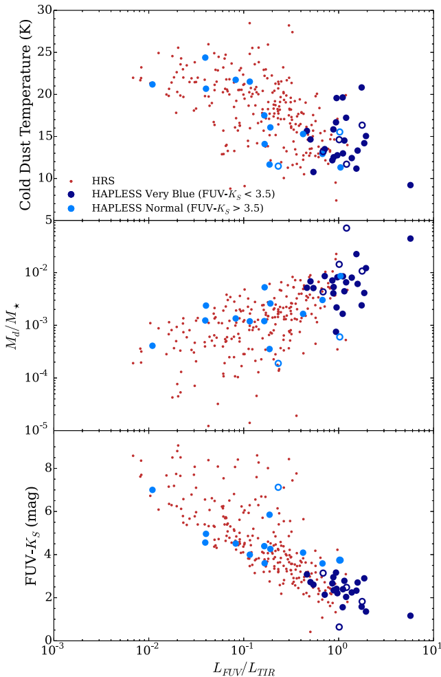
Figure 15. Scaling relations with L_{\text{FUV}}/L_{\text{TIR}} for the HAPLESS and HRS. Upper: cold dust temperature against L_{\text{FUV}}/L_{\text{TIR}} . Centre: M_d/M_* against L_{\text{FUV}}/L_{\text{TIR}} ; counter-intuitively, the more dust-rich a galaxy, the larger the proportion of FUV photons that go unabsorbed. Lower: FUV- K_S colour against L_{\text{FUV}}/L_{\text{TIR}} ; correlation is very tight for bluer galaxies, but far weaker for redder galaxies.
