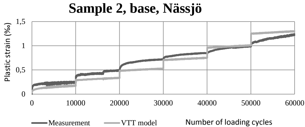
Figure 4. An example of regression factor calibration (Sample 2, base, Nässjö).
