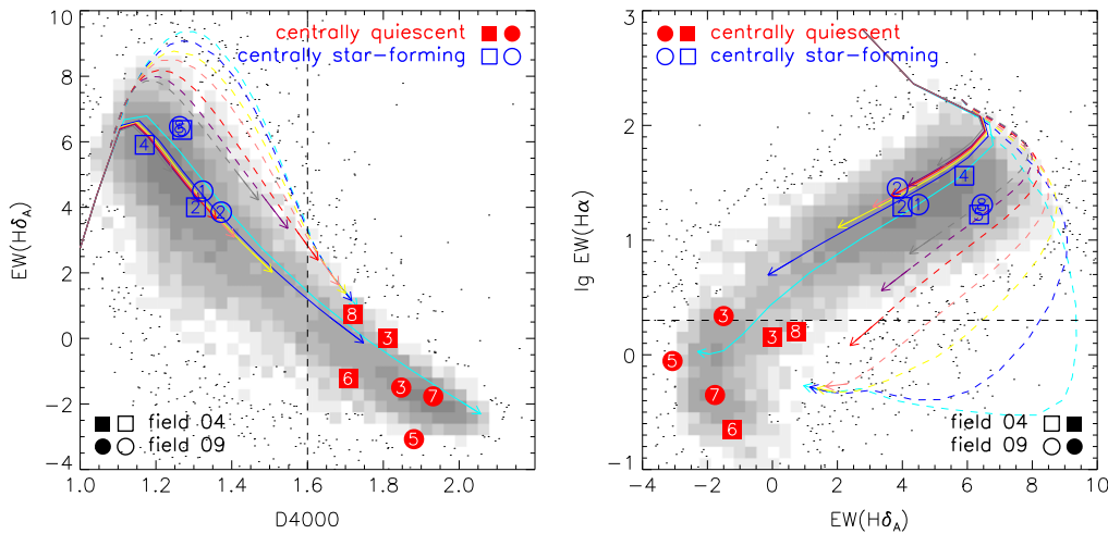
Figure 2. P-MaNGA galaxies are plotted as large red or blue symbols on planes of 4000 Å break vs. H\delta_A (left panel) and H\delta_A vs. \log_{10}EW(H\alpha) (right panel). Shown by solid and dashed lines are solar-metallicity models of continuous star formation histories and star formation bursts calculated using the stellar population synthesis code of Bruzual & Charlot (2003). Distributions of a volume-limited sample selected from the SDSS are shown as gray scale for comparison. Symbols/colors are the same as in the previous figure. The dashed vertical line in the left panel indicates a constant D_n(4000) = 1.6 , while the dashed horizontal line in the right panel is for EW(H\alpha) = 2 \text{ \AA} ; these are the typical values adopted in the literature to divide a galaxy into quiescent and star-forming populations.
