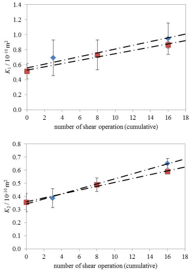
Figure 12. Experimentally determined principal permeability values, K_1 and K_2 , for a 2×2 twill weave fabric with S_0 = 660 \text{ g/m}^2 , fibre volume fraction V_f = 0.56 , after undergoing different shear operations; diamond symbols: specimens clamped parallel to warp direction during shear; square symbols: specimens clamped parallel to weft direction during shear; error bars indicate standard deviations.
