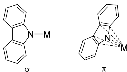
Figure 2. Schematic representation of monohapto \sigma -bonding and multihapto \pi -bonding modes of carbazolyl ligands.
