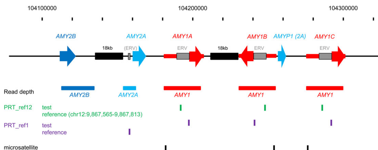
Figure 1. General overview of the human amylase gene region, showing the positions of assays used. The corresponding region of the human reference (hg19) assembly shown includes three copies of AMY1 (AMY1A/1B/1C) and one copy each of AMY2A and AMY2B. In each case, the broad arrow indicates the position and orientation of the gene, and the more extensive region of near-perfect sequence identity around each copy of AMY1 is shown as a narrower red rectangle. Exons 4–10 of AMY2A are repeated in the truncated pseudogene AMYP1 between AMY1B and AMY1C. The black '18 kb' rectangles indicate two near-identical regions with multiple sequence similarity to other parts of the locus. The 'read-depth' annotation shows the regions used for read-depth analysis of AMY2B (dark blue), AMY2A (light blue) and AMY1 (red), indicating coherent intervals not compromised by high-sequence identity to other locations. The 'PRT_ref12', 'PRT_ref1' and 'microsatellite' annotations indicate the predicted positions of PCR products used in our copy number measurements at this locus.
