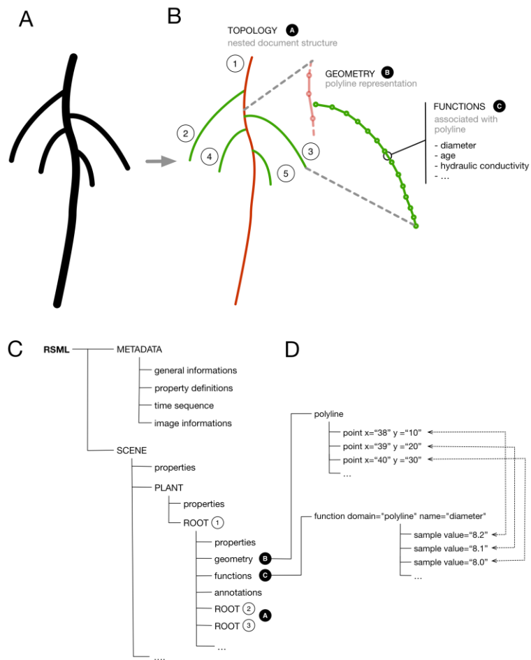
Figure 2: visual representation of the RSML structure. A. Original image B. Graphical representation of the structure. Topology (primary root in red and lateral roots in green), geometry and properties are represented at different levels. C. Schematic representation of an RSML file structure. D. Representation of the coupling between the root geometry and its associated functions (here the diameter). Dotted lines represent data from the same point in a polyline.
