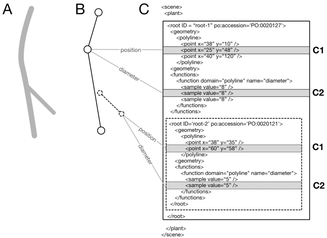
Supplemental figure 1: RSML representation. A. Example root system. B. Representation of the roots as polylines. The plain line represent the primary root while the dotted line represent the lateral root. C. Corresponding RSML structure (only the scene section). The plain-line box represents the domain of the primary root. The dotted-line box represents the domain of the lateral root. The nested structure of the RSML format represent the topological relations between the different roots. In this example, each points of the polylines (B) is represented by its position in the image (C1) and its diameter (C2).
