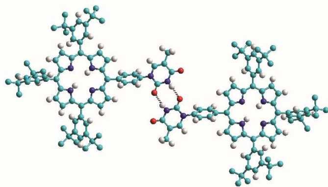
Figure 2. View of the single crystal X-ray structure of mono-TP illustrating the formation of the inter-thymine R^2_2(8) double hydrogen-bonding interaction (represented with the two dotted lines) observed in the solid state. Hydrogen atoms of the tert-butyl groups are omitted for clarity. Atoms are colored as follows C - light blue; N - dark blue; H - white; O - red.
