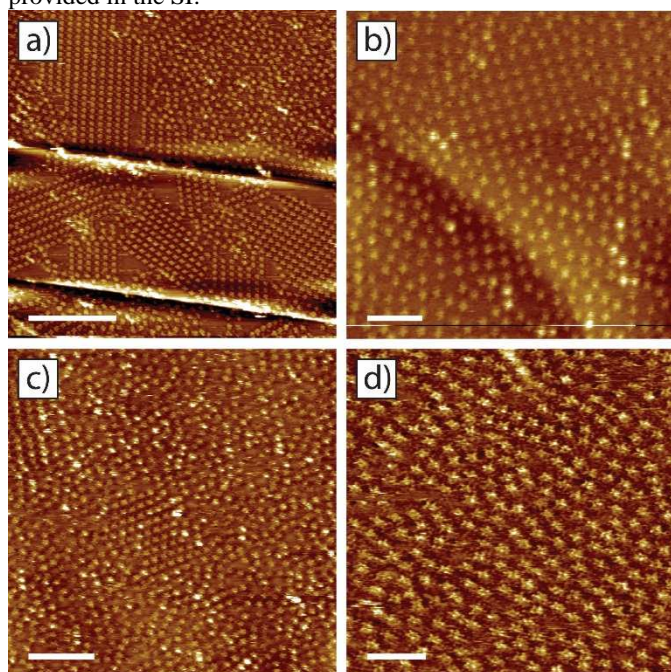
Figure 6 Influence of the concentration and molar ratio of components on the morphology of the tetra-TP / 9-propyladenine network. a) Tetra-TP ( 1.41 \times 10^{-5} \text{ M} ) and 9-propyladenine ( 2.26 \times 10^{-4} \text{ M} ) mixture: molar ratio 1:16. b) Tetra-TP ( 3.03 \times 10^{-5} \text{ M} ) and 9-propyladenine ( 8.07 \times 10^{-6} \text{ M} ) mixture: molar ratio 4:1. c) Tetra-TP ( 1.77 \times 10^{-5} \text{ M} ) and 9-propyladenine ( 1.13 \times 10^{-3} \text{ M} ) mixture: molar ratio 1:64. d) Tetra-T-porphyrin ( 5.04 \times 10^{-6} \text{ M} ) and propyl adenine ( 1.93 \times 10^{-3} \text{ M} ) mixture: molar ratio 1:383. STM imaging parameters: V_s = -0.5 \text{ V} ; I_t = 15 \text{ pA} . Scale bars: a) 40 nm; b) 10 nm; c) 20 nm; d) 10 nm.
