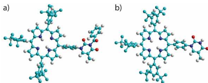
Figure 1. Single crystal X-ray structures of (a) benzoyl-mono-TP and (b) mono-TP. Note the relative orientation of the thymine moiety with respect to the porphyrin plane. Hydrogen atoms of the tert-butyl groups are omitted for clarity. Atoms are colored as follows C - light blue; N - dark blue; H - white; O - red.
