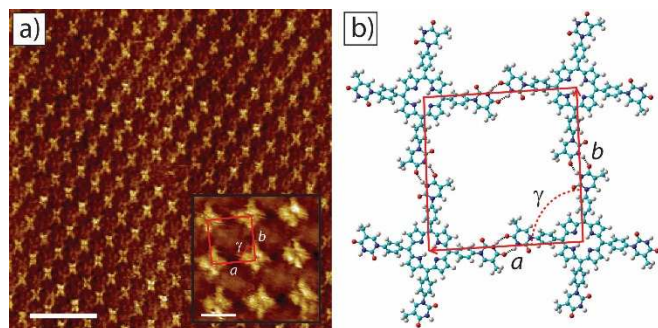
Figure 4. 2D self-assembled network of tetra-TP at the TCB-HOPG liquid-solid interface. a) Large scale STM image of the tetra-T-porphyrin ( 2.82 \times 10^{-5} M) network at the TCB-HOPG liquid-solid interface. The insert shows a high resolution, drift corrected STM image of the network with an individual 2D unit cell marked in white: unit cell parameters a = 25.9 \pm 0.5 Å; b = 25.2 \pm 0.6 Å; and \gamma = 91 \pm 1^\circ . STM imaging parameters: V_s = -0.5\text{V} ; I_t = 15\text{pA} . Scale bar = 20nm (insert = 2nm). b) Molecular model of the tetra-T-porphyrin network from MM simulations. Unit cell parameters a = 26.0 Å; b = 25.9 Å; and \gamma = 90^\circ .
