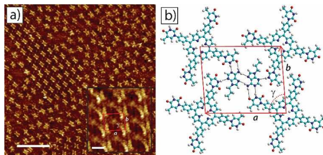
Figure 5. 2D self-assembled network of tetra-TP and 9-propyladenine at the TCB-HOPG liquid-solid interface. a) Large scale STM image of the tetra-TP ( 2.82 \times 10^{-5} M) and 9-propyladenine ( 4.52 \times 10^{-4} M) network at the TCB-HOPG liquid-solid interface. The insert shows a high resolution, drift corrected STM image of the network with an individual 2D unit cell marked in red: unit cell parameters from STM images a = 25.4 \pm 0.7 Å; b = 22.2 \pm 0.9 Å; and \gamma = 83 \pm 2^\circ . STM imaging parameters: V_s = -0.5\text{V} ; I_t = 15\text{pA} . Scale bar = 200 Å (insert = 16 Å). b) Molecular model of the tetra-T-porphyrin network from MM simulations. Unit cell parameters from MM simulations a = 26.0 Å; b = 21.5 Å; and \gamma = 85.7^\circ .
