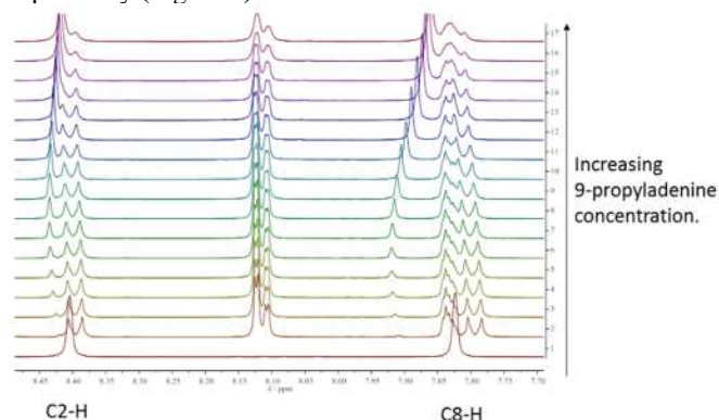
Figure 3. 1 H NMR spectrum illustrating shifts in the C8-H and C2-H proton signals during titration of mono-TP with 9-propyladenine. Spectrum 1 corresponds to pure 9-propyladenine and spectra 2-17 are recorded with constant mono-TP concentration and increasing 9-propyladenine concentration.
