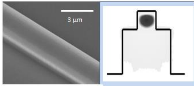
Fig. 2: Scanning Electron Microscopy image (left) of 2.5 μm wide waveguide using Inductively-Coupled Plasma etching SiCl 4 / Ar at a substrate temperature of 0°C and simulation (right) using Optiwave of single-mode, polarization-maintaining waveguide in cross-section for 780 nm laser light
