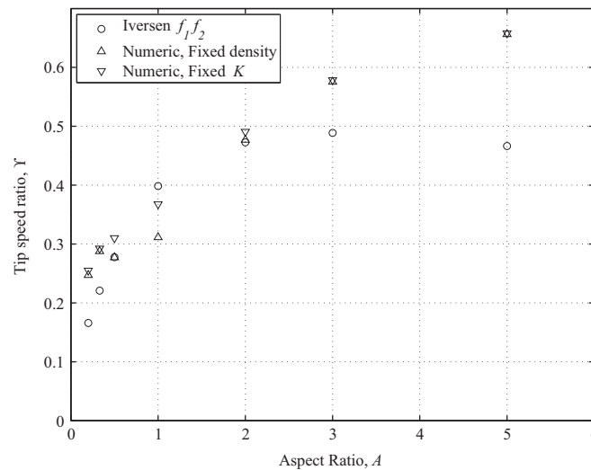
Fig. 22. The variation of the tip speed ratio, Y , with aspect ratio, A , for plates of low and high moment of inertia parameter, K , as predicted by the Iversen (1979) correlations and the numerical simulations.
