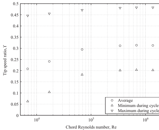
Fig. 24. The variation of the tip speed ratio, Y , with the Reynolds number, Re , for aspect ratio, A=1 , thickness ratio, \tau=0.0254 and moment of inertia parameter, K=0.1838 .
