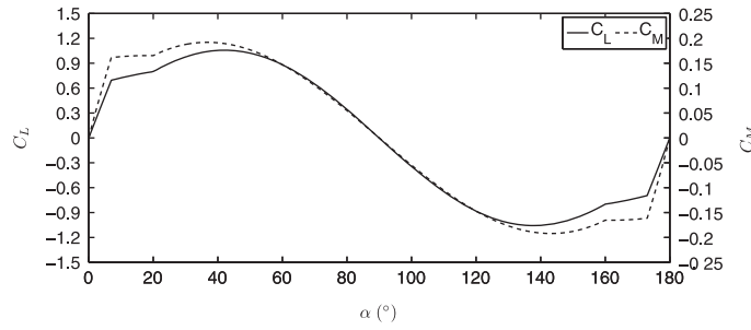
Fig. 1. Steady-state curves showing the variation of lift, C_L , and moment, C_M , coefficients with angle of attack, \alpha for static square flat plates held in a uniform steady flow (ESDU, 1970).
