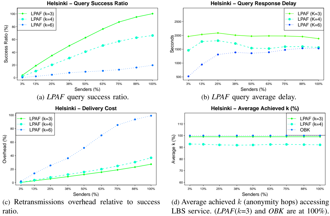
Fig. 7: Comparison of LPAF performance for different privacy-level requirements ( k ) and using various ratio of senders.
