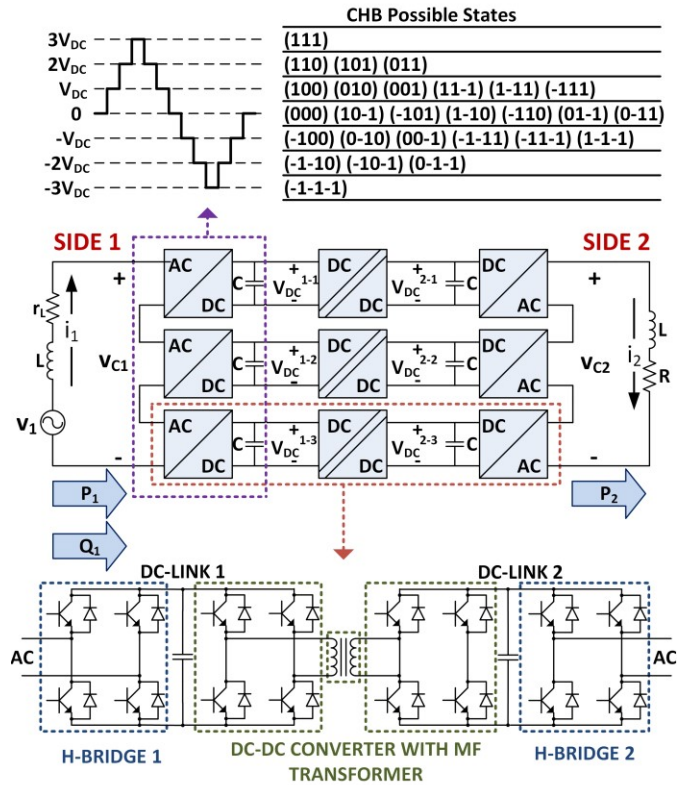
Fig. 1. Converter schematic (center) with detailed schematic of the single cell (bottom) and description of the switching patterns (top).
