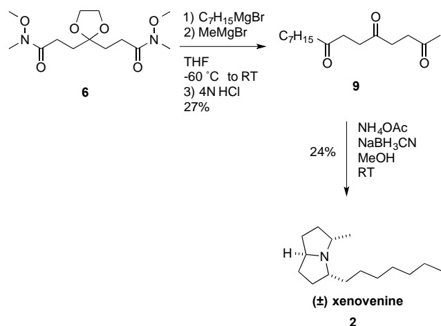
Scheme 3. Synthesis of xenovenine
