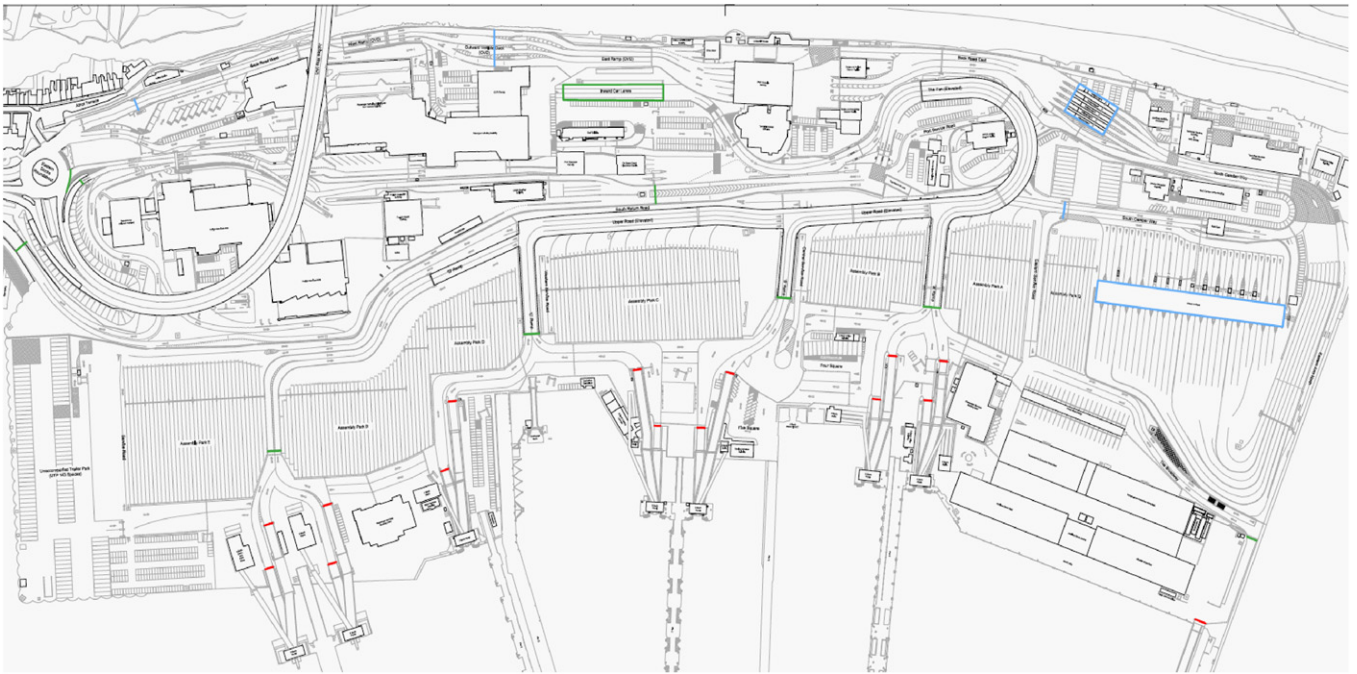
Fig. 1. Plan of the Port of Dover.
