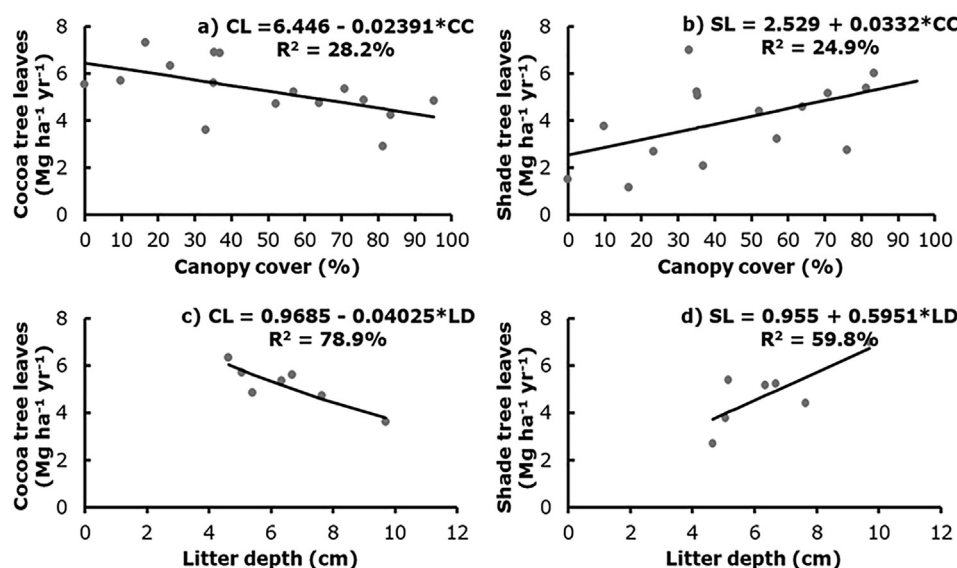
Figure 8. Relationship between selected stand parameters of smallholder cocoa systems at Suhum. Panel a) annual cocoa leaf litter (CL, \text{Mg ha}^{-1} \text{yr}^{-1} ) and canopy cover (CC, %), panel b) annual leaf litter of shade trees (SL, \text{Mg ha}^{-1} \text{yr}^{-1} ) and canopy cover, panel c) litter depth (LD, cm) and cocoa leaf litter, and panel d) litter depth and leaf litter of shade trees. The relationship between litter depth and cocoa and shade tree leaves (panels c and d) was assessed in organic farms.
