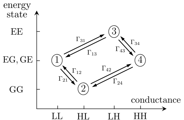
FIG. 4. Stochastic system of the two molecules: the four possible states and connecting transitions.
