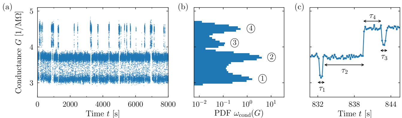
FIG. 2. (a) Conductance as function of time. (b) Probability density function PDF of the conductance values. Four different molecular states give rise to four maxima. (c) Segment of the conduction time trace from (a). Individual jumps between the conductance plateaus are visible. Lifetimes can be identified as indicated by \tau_1, \tau_2, \tau_3 , and \tau_4 . The authors gratefully acknowledge re-use of the data from Ref. [26], Copyright © 2020 American Chemical Society.
