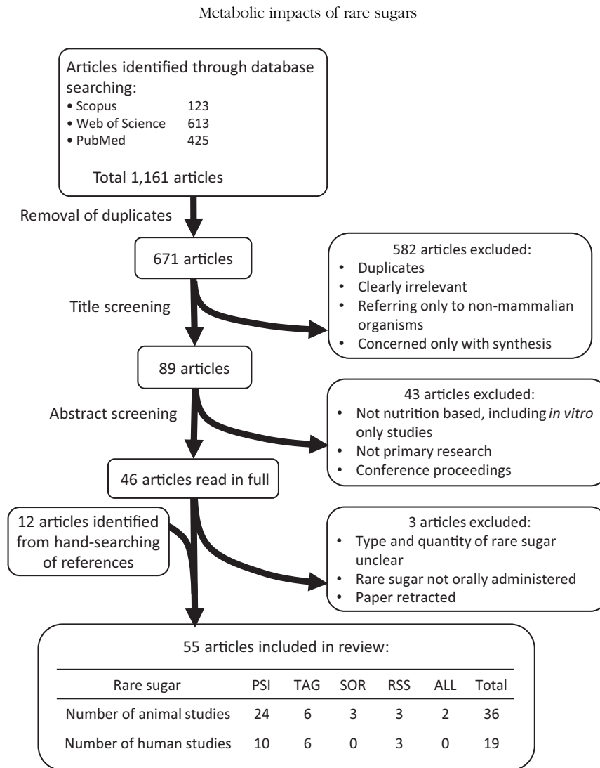
Fig. 1 Identification and selection of relevant research. PSI: D-psicose, TAG: D-tagatose, SOR: D-sorbose, RSS: rare sugar syrup, ALL: D-allose.
