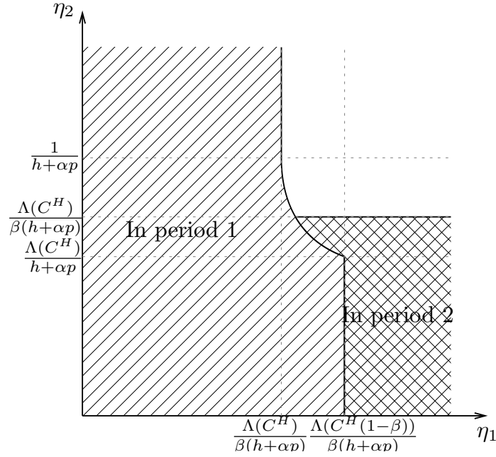
Figure 9: Probability of purchasing in period 1 and 2 when shopping costs are high both periods and discount factor is high.
