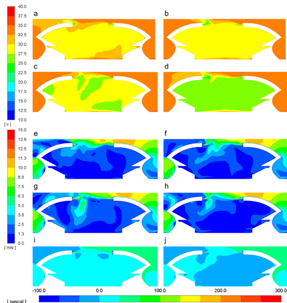
Figure 10. (a–d) Temperature contours of the cross-section of the stadium for scenarios one to four. (e–h) Wind velocity contours of the cross-section of the stadium for scenarios one to four. (i,j) Total pressure contours of the cross-section of the stadium for scenarios three to four.
