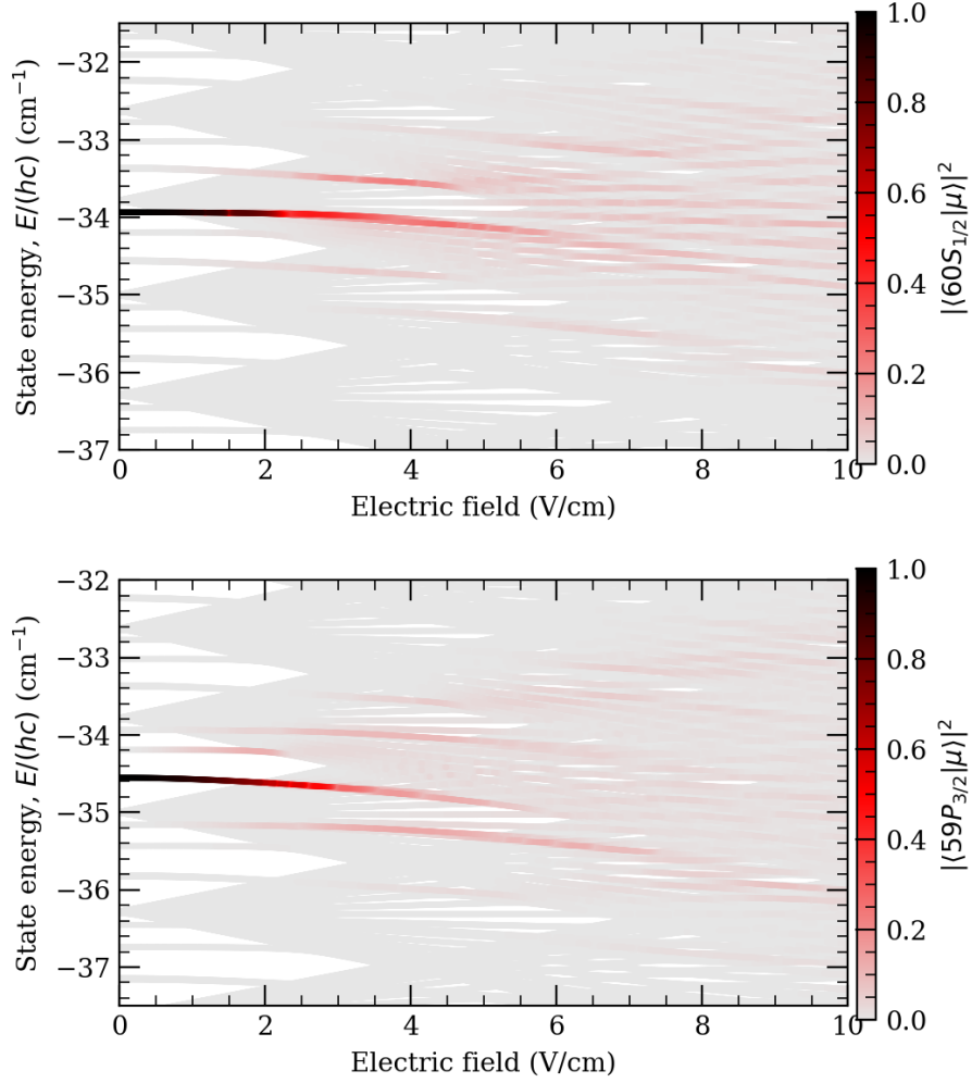
Figure S3: Stark shifts of the 60S_{\frac{1}{2}}, 59P_{\frac{3}{2}} energy level of Rubidium. The stark effect is only quadratic for small E_0 . Divergence from a simple E^2 relationship begins at around around E_0 = 2 V/cm, and is clearly present at E_0 = 4 V/cm for both states. This effect can be seen in the divergence of the observed fringe visibility from the quartic model of figure (S2).
