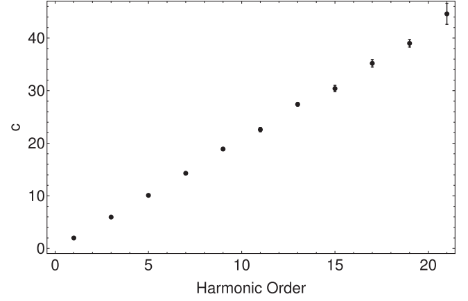
FIG. 5. Our numerical results for the mean value of the cusps per period c , with harmonic order from 1 to 21.
