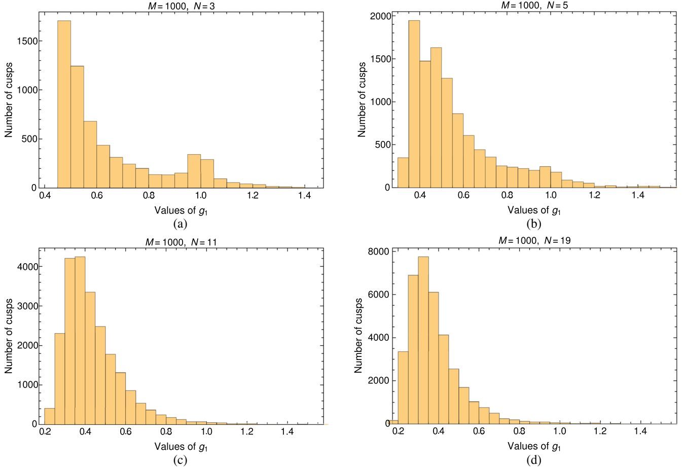
FIG. 6. The frequency distribution of the parameter g_1 calculated for different harmonic orders. Note that the data originate from a representative sample of M = 1000 cosmic string loops for each plot. We can see that the total number of cusps increases with the harmonic order, which is expected since the average number of cusps per period for each loop also increases with the harmonic order. Note that we have cut some rare higher values of g_1 from the histograms. The maximum value of g_1 in the data is given in Table.
