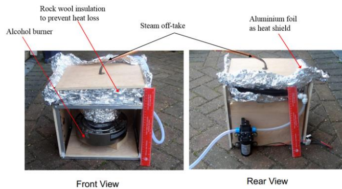
Figure 4. Flash boiler experimental test rig
