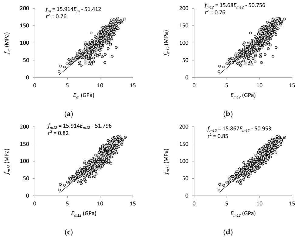
Figure 5. Correlation between modulus of elasticity ( E_m ) and bending strength ( f_m ). (a) With the moisture content at the time of the tests (Phase 1); (b) After the correction for a 12% of moisture content (Phase 2); (c) After excluding the outliers (Phase 3); (d) After excluding 5% of the values farthest from the linear regression expression.
