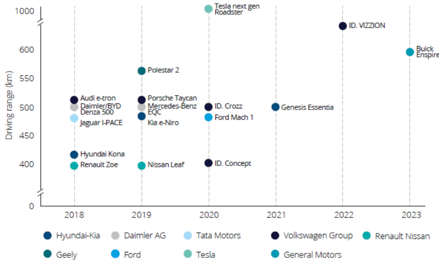
Fig. 4 The driving range for the next generation BEVs [13]
