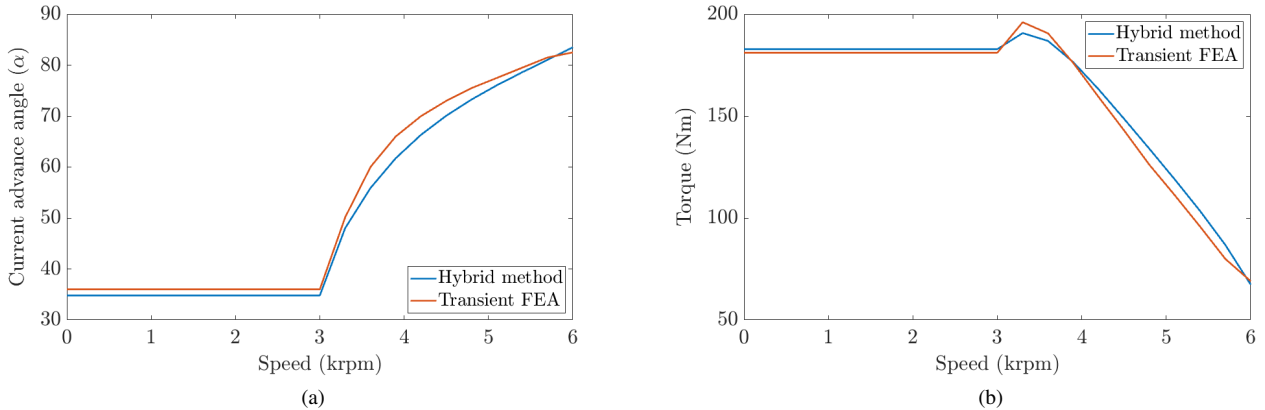
Fig. 5. Comparison between hybrid method and transient FEA for machine 3 using (a) current advance angle and (b) complete torque-speed characteristics
