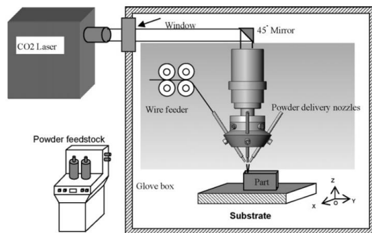
Figure 19: Schematic of a DED system with simultaneous powder and wire feed. [320]
