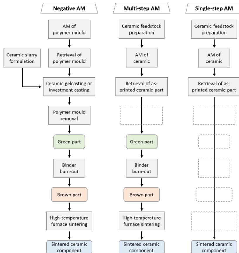
Figure 5: Flowchart showing the number of steps of negative ceramic AM, multi-step direct AM, and single-step direct AM, from AM feedstock to sintered ceramic part.
