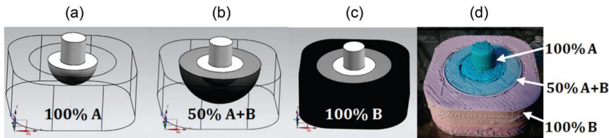
Figure 10: Functionally graded material part fabricated using two \text{CaCO}_3 pastes. [187]
