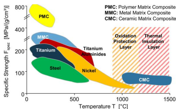
Figure 6: Specific strength of materials as a function of working temperature for turbomachinery components. [55]
