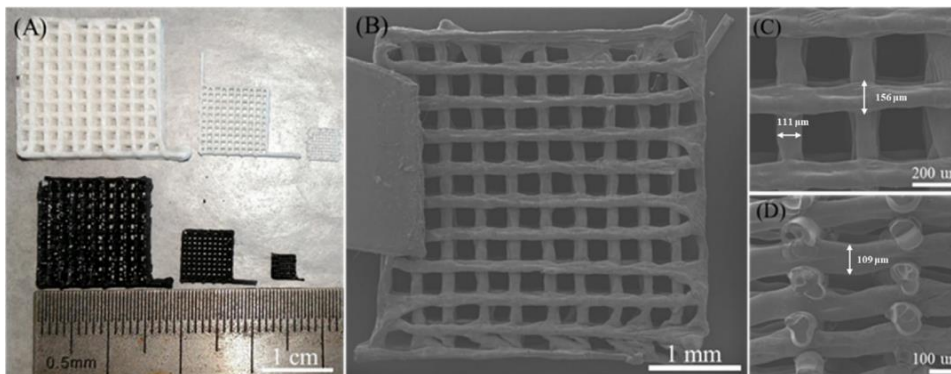
Figure 8: (A) 3D scaffolds (16 layers) assembled from PCS/n-hexane solutions deposited through 400 µm, 200 µm and 100 µm nozzle respectively, before (white) and after (black) pyrolysis. (B to D) SEM images of 3D SiC scaffold assembled through 100 µm nozzle: top view (B-C) and side view (D).
