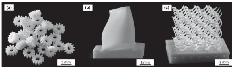
Figure 15: Sintered alumina parts fabricated using the LCM technique: (a) gear wheels; (b) a turbine blade; and (c) a cellular cube. [280]
