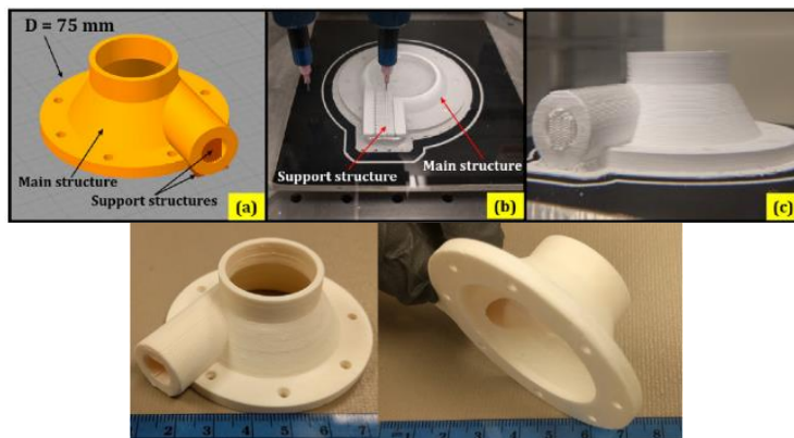
Figure 11: TOP: Sample turbine-blower housing: (a) CAD model with main and support structures, (b) part being printed, (c) completely printed part surrounded by oil. BOTTOM: Final turbine-blower housing part after removal of support and sintering. [188]
