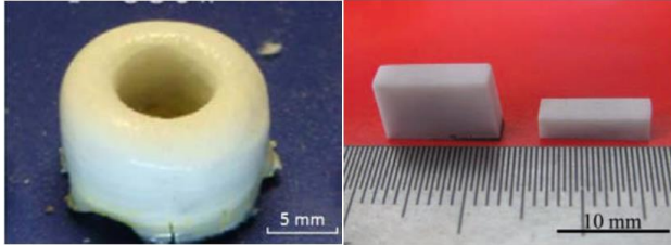
Figure 20: Hollow cylinder structure fabricated by LENS (LEFT) and rectangular samples machined from the fabricated specimen (RIGHT). [324]
