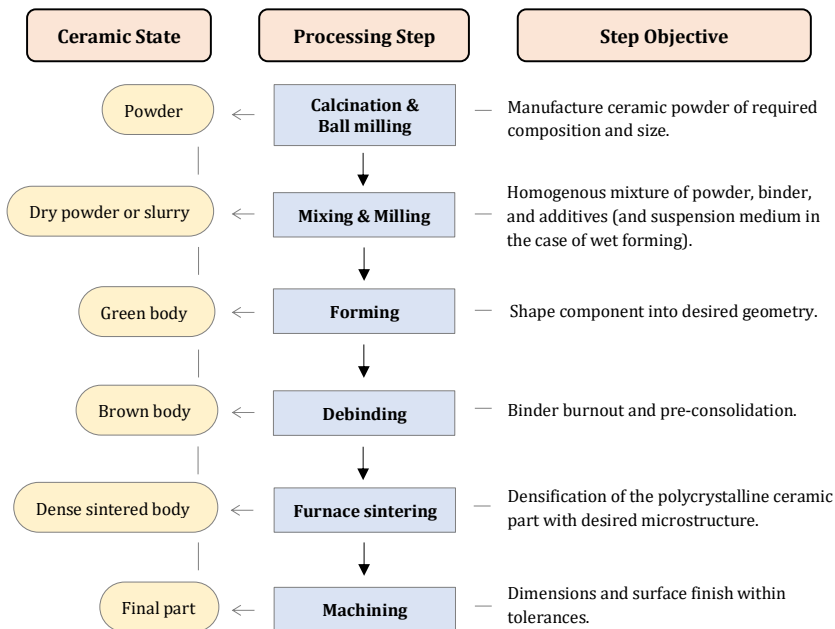
Figure 1: Flowchart for the ceramic powder processing route from starting powder to final part.
