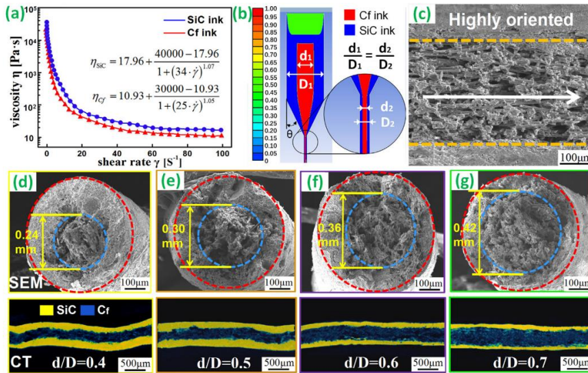
Figure 9: (a) Shear rate-dependent viscosity and fitting curve based on the Cross model and (b) Numerical simulation of the co-extrusion process. (c) Cf were highly oriented in the direction of extrusion. (d–g) SEM and CT of Core-Shell filaments with a d/D ratio from 0.4 to 0.7, respectively. [180]
