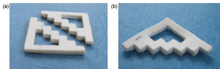
Figure 7: LZSA laminates in stair-like geometry produced by LOM in the green state (a) and after sintering (b). [104]
