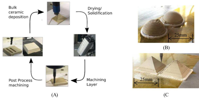
Figure 13: Process flow for the hybrid additive-subtractive manufacturing of ceramics (A). The surface finish of 3D printed components is significantly improved when using the hybrid manufacturing approach, as demonstrated by hollow hemispheres (B) and pyramids (C) [197]
