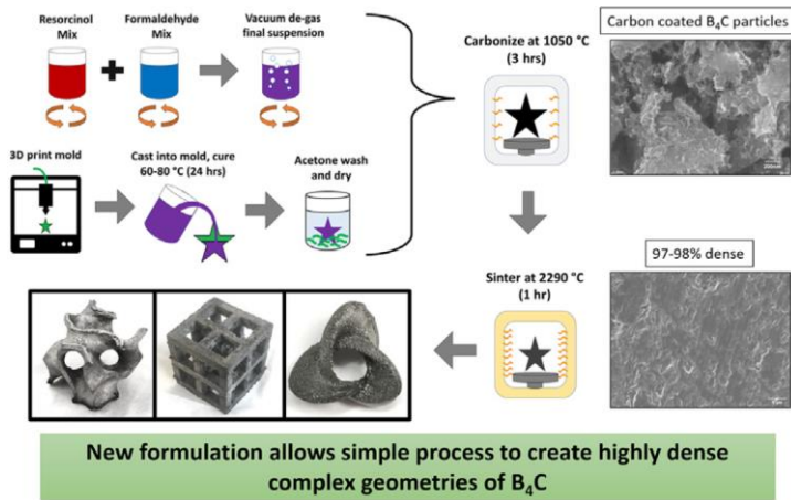
Figure 4: Negative additive manufacturing processes based on gelcasting to create complex B_4C components. [22]
