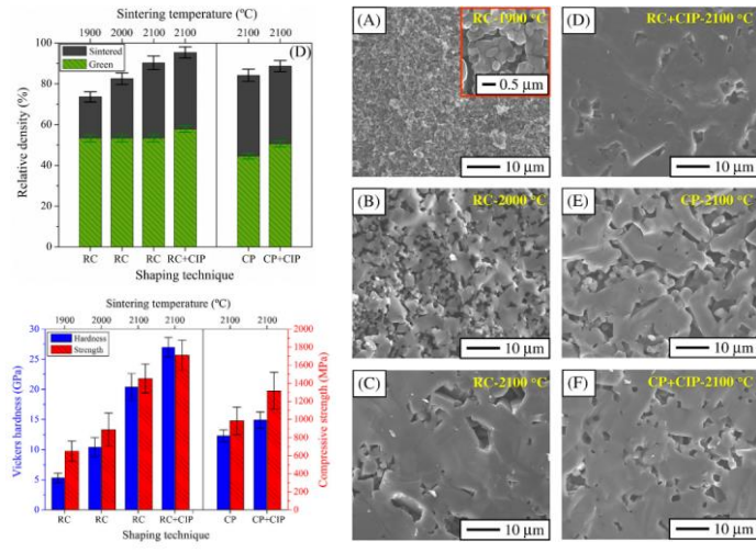
Figure 22: Effect of SPS firing temperature and of CIP on the density and mechanical properties of sintered B_4C samples produced by robocasting. [161]
