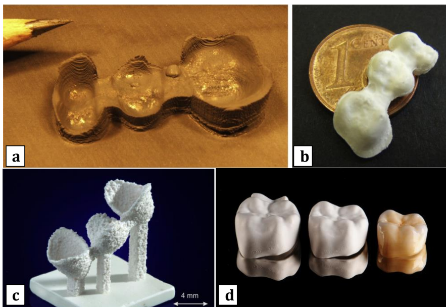
Figure 21: Comparison of dental crowns and frameworks produced using a number of AM technologies. A supportive base made of carbon black (a) and the corresponding sintered 3Y-TZP bridge framework (b) produced using DIP, showing an appreciable surface finish despite some surface defects caused by the support materials [228]. D ental restoration frameworks manufactured by dLS have a very high surface roughness (c) [311], while dental crowns made by DLP (d) display an excellent surface finish and a high level of detail, from the as-printed state to the stained and sintered state (image provided as a courtesy by Dr Johannes Homa, CEO of Lithoz GmbH).
