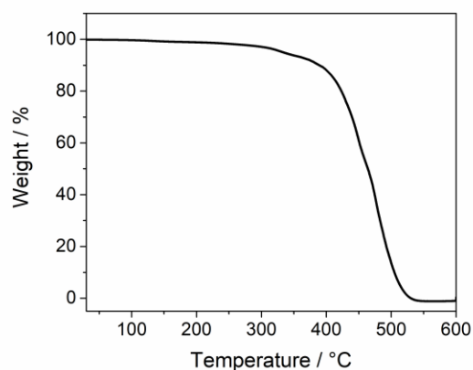
Figure S-2: TGA trace of FS-5Dodec powder heated at 10\text{ }^{\circ}\text{C min}^{-1} under air.
