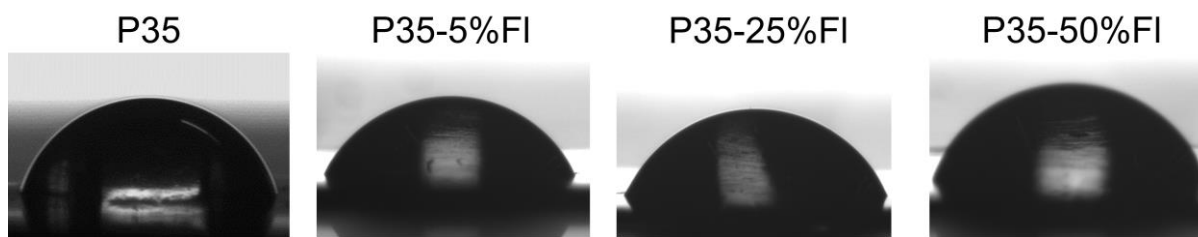
Figure S-30: Water drops on films of P35 and the P35 fluorenone co-polymers . Contact angles were measured to be 77 \pm 3^\circ for P35, 72 \pm 3^\circ for P35-5%FI, 78 \pm 1^\circ for P35-25%FI, and 83 \pm 2^\circ for P35-50%FI. Small differences could originate in grain-sizes on the surface of the pressed pallets.
