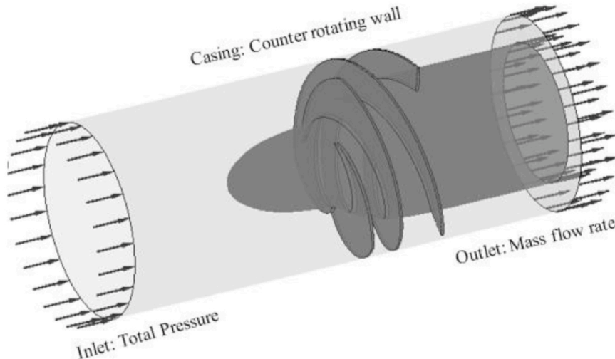
Fig. 2. Computational domain of the studied inducer.
