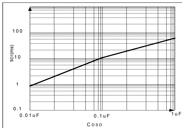
t_{D1} VS C_{DSD}
