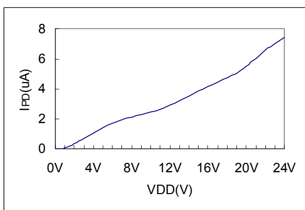
I_{PD} VS V_{DD}
