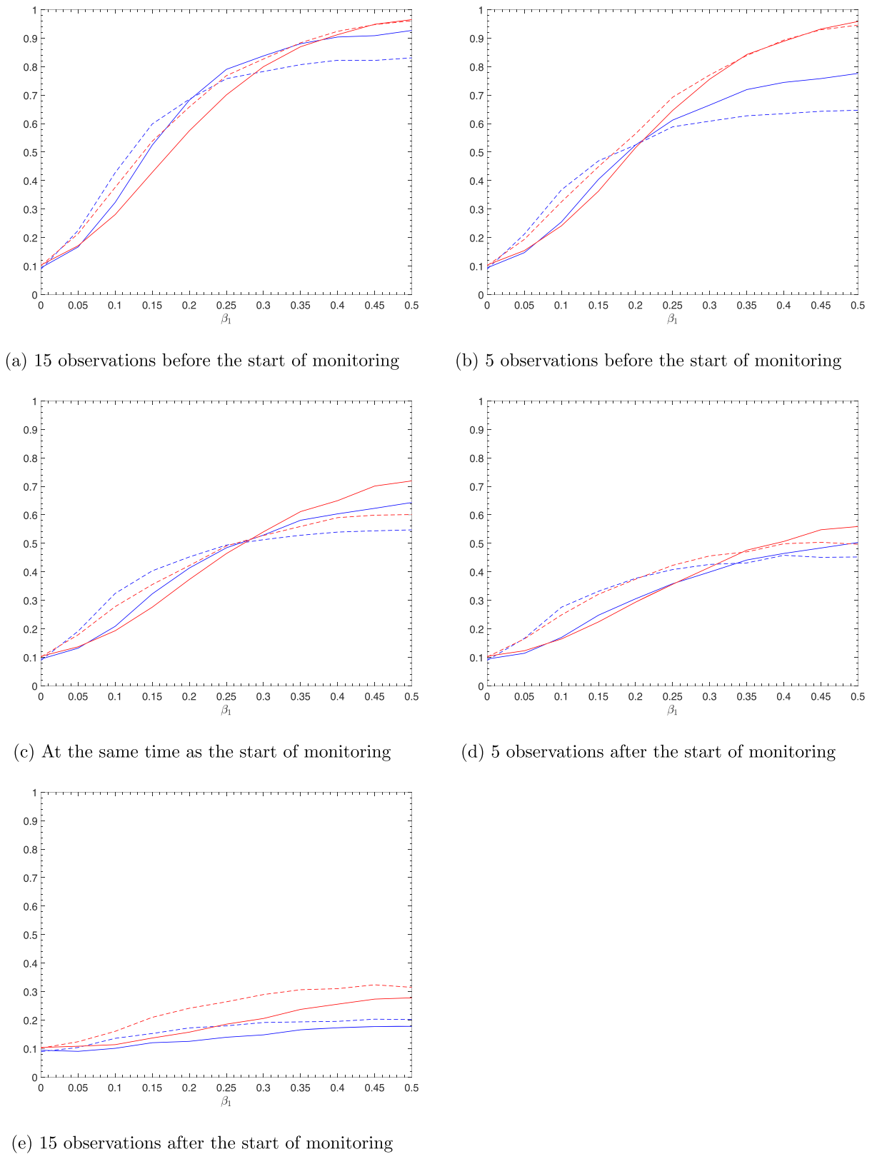
FIGURE 2 Predictive regime detection frequency as a function of \beta_1 for different values of \rho : T^* + m = 302 , E = 327 , m_1 = 30 , m = 30 ; MAX, \rho = 0.965 , —; MAX, \rho = 0.995 , - -; SEQ, \rho = 0.965 , —; SEQ, \rho = 0.995 , - - [Colour figure can be viewed at wileyonlinelibrary.com ]
