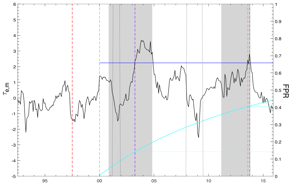
FIGURE 8 lt_{t-1} , MAX procedure, m = 30 : — ( \tau_{e,m} ), — ( \max_{e \in [m+1, T^*]} \tau_{e,m} ), - - - ( T^* ), - - - ( T^* + m ), - - - (first rejection), - - - (second rejection), - - - (third rejection), ■ (weak set of dates), — (false positive rate), ····· (NBER indicator) [Colour figure can be viewed at wileyonlinelibrary.com ]
