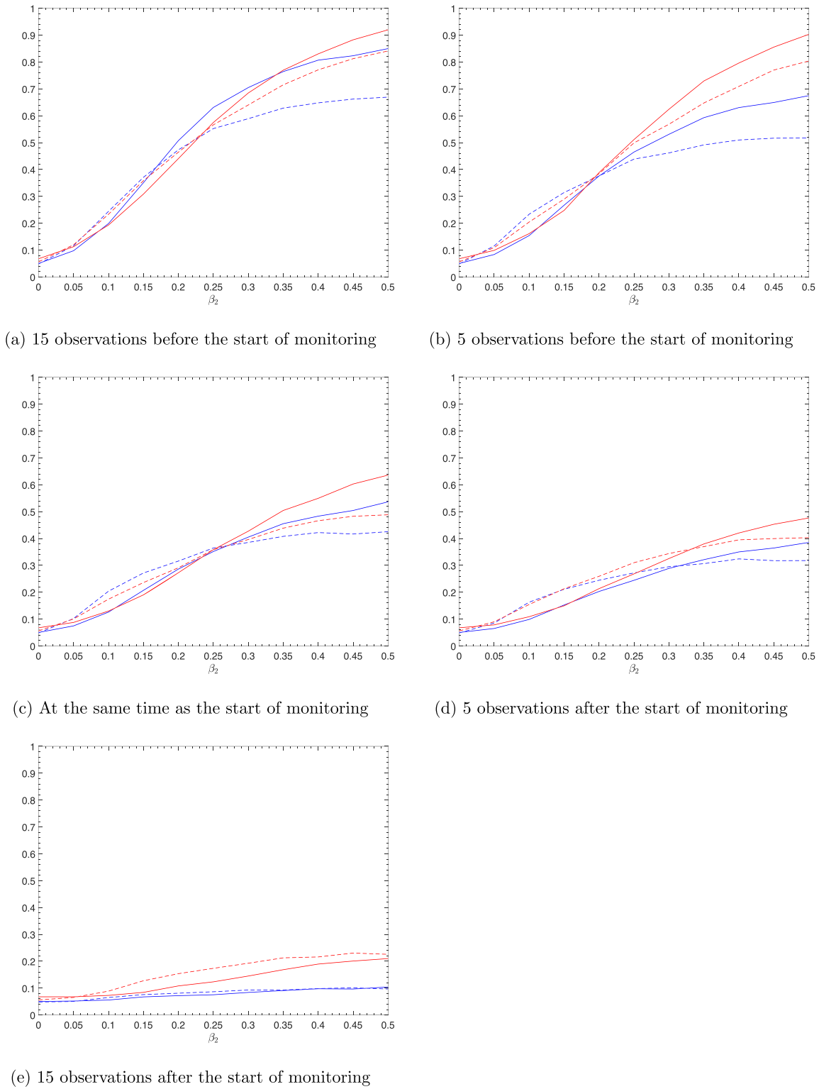
FIGURE 4 Detection frequency for a second predictive regime when a predictive regime with \beta_1 = 0.25 also exists in the training period, as a function of \beta_2 for different values of \rho : T^* + m = 302 , E = 327 , m_1 = 15 , m_2 = 30 , m = 30 ; MAX , \rho = 0.965 , —; MAX , \rho = 0.995 , - - -; SEQ , \rho = 0.965 , —; SEQ , \rho = 0.995 , - - - [Colour figure can be viewed at wileyonlinelibrary.com ]
