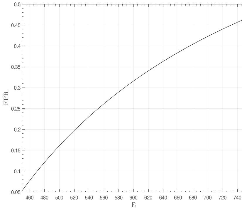
FIGURE 1 FPR as a function of E
