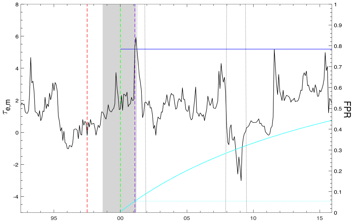
FIGURE 6 dp_{t-1} , MAX procedure, m = 30 : — ( \tau_{e,m} ), — ( \max_{e \in [m+1, T^*]} \tau_{e,m} ), - - - ( T^* ), - - - ( T^* + m ), - - - (first rejection), ■ (weak set of dates), — (false positive rate), ···· (NBER indicator) [Colour figure can be viewed at wileyonlinelibrary.com ]
