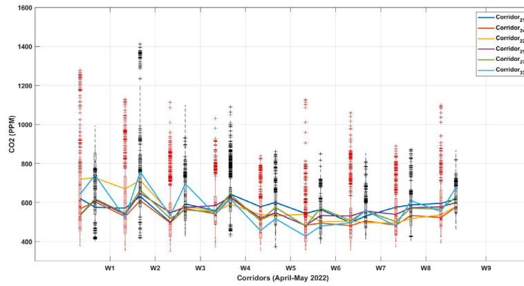
(a) CO 2
