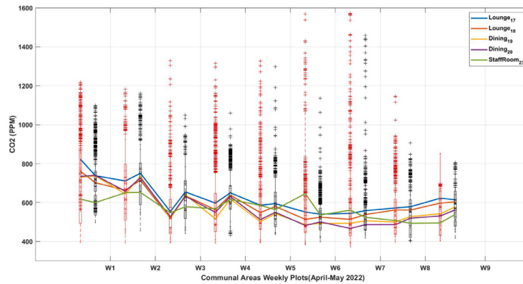
(a) CO 2
