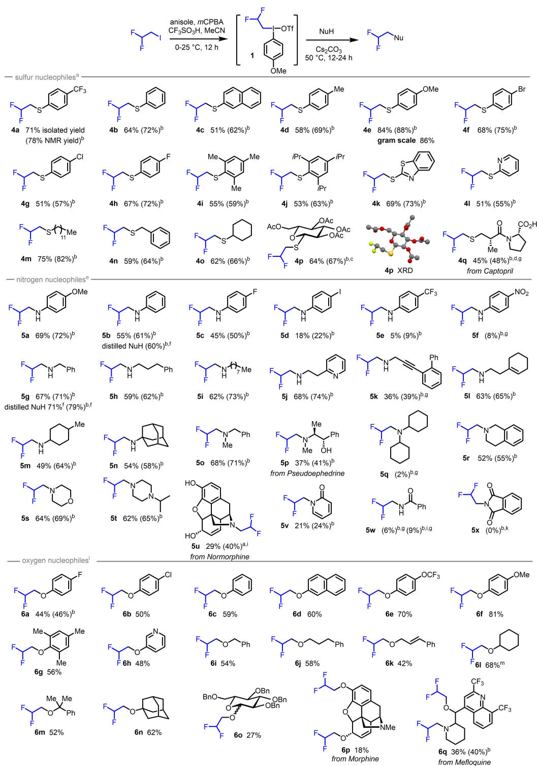
Scheme 2. 2,2-Difluoroethylation Scope. [a] Reaction conditions for thiol nucleophiles: (i) 1,1-difluoro-2-iodoethane (1.04 mmol), anisole (1.1 equiv.), mCPBA (2.5 equiv.), CF 3 SO 3 H (1.2 equiv.), MeCN (5 mL, 0.2 M), 0–25 °C, 12 h; (ii) thiol (1.1 equiv.), Cs 2 CO 3 (2.0 equiv.), 50 °C, 12 h. Yields are of isolated products. [b] Crude yield in parentheses, determined by 19 F NMR spectroscopy using trifluorotoluene as internal standard. [c] Structure confirmed by XRD. [d] Reaction time (step 2) = 36 h. [e] Reaction conditions for amine nucleophiles: (i) 1,1-difluoro-2-iodoethane (1.04 mmol), anisole (1.1 equiv.), mCPBA (2.1 equiv.), CF 3 SO 3 H (1.2 equiv.), MeCN (5 mL, 0.2 M), 0–25 °C, 24 h; (ii) amine (1.5 equiv.), Cs 2 CO 3 (2.0 equiv.), 50 °C, 24 h. Yields are of isolated products. [f] The amine nucleophile was distilled before use. [g] NaH (3.5 equiv.) was used as the base in step 2. [k] No reaction with phthalimide or potassium phthalimide; reaction time (step 2) = 3 days. [l] Reaction conditions for alcohol nucleophiles: (i) 1,1-difluoro-2-iodoethane (1.04 mmol), anisole (1.1 equiv.), mCPBA (2.5 equiv.), CF 3 SO 3 H (1.2 equiv.), MeCN (5 mL, 0.2 M), 0–25 °C, 24 h; (ii) alcohol (1.5 equiv.), NaH (3.5 equiv.), 50 °C, 24 h. Yields are of isolated products. It was not possible to report crude yields for most of these reactions, as the ether products 6 were indistinguishable from by-product 5 by 19 F NMR. [m] Reaction time (step 2) = 16 h.
