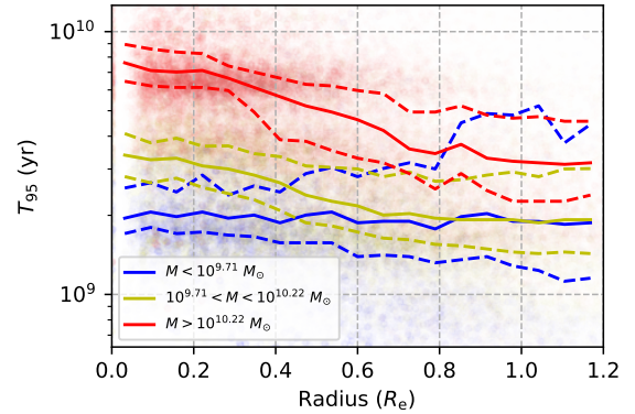
Figure 5. Time since 95% of the stellar mass built up ( T_{95} ) in each spaxel of each galaxy in the spiral sample. Each spaxel in each galaxy is shown as a point, with the opacity defined by the product of the total spaxel flux and the galaxy’s MaNGA Primary+ sample weight. Colours denote the galaxy’s total present-day mass. Solid lines represent a weighted running median, and dashed lines are one-third and two-third weighted percentiles. The outskirts of galaxies of all masses built up at approximately similar times, but the centres of massive galaxies formed significantly earlier than those of low-mass galaxies. The apparent horizontal feature in the high-mass data points at \sim 7 Gyr is an artefact: there’s a large number of spaxels which have not reached T_{95} by 8.9 Gyr but have by the next oldest SSP at 4.5 Gyr, causing an apparent cluster between these two ages.
