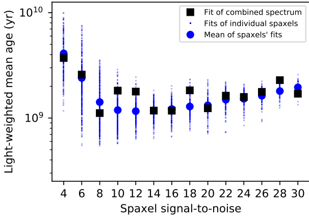
Figure A1. The mean age of spaxels in different signal-to-noise ratio bins ( blue ) in a spiral galaxy compared to the mean age of the spectrum of all spaxels combined ( black squares ). There is no significant bias in the average age measured by STARLIGHT compared with varying SNR.
