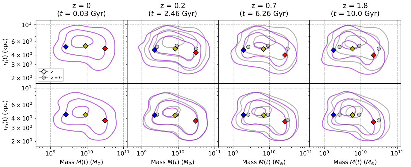
Figure 10. The distributions of galaxies at individual snapshots in Figure 9 showing the mass– r_1 ( upper panels ) and mass– r_m ( lower panels ) planes at selected redshifts z . The corresponding lookback times t are also indicated. As fiducials, the grey contours and circle markers indicate the distribution of galaxies and the mean positions of each mass bin at z = 0 , while the magenta contours and coloured diamond points indicate the distribution and mean positions at each redshift’s time slice.
