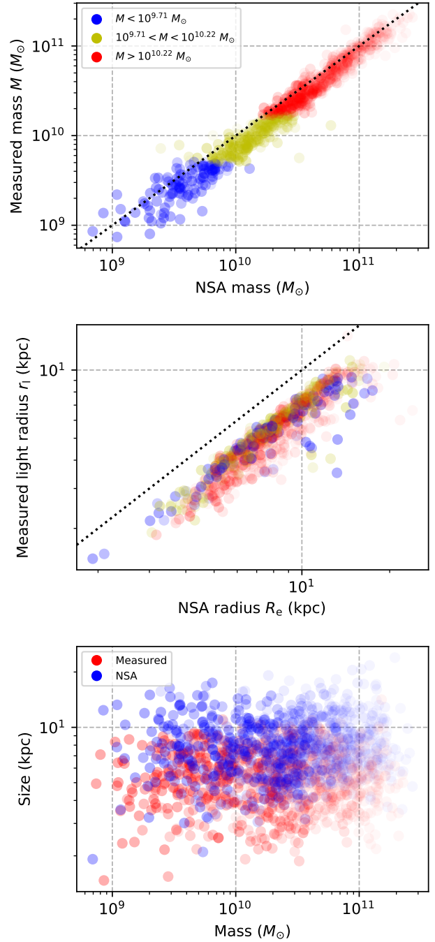
Figure 8. Comparison of the masses ( top ) and radii r_1 ( middle ) of the spiral sample taken from the NASA-Sloan Atlas (?) and measured by STARLIGHT within 1.2 R_e . The dashed lines indicate equality. Both measurements are consistent with the NSA values, with the offset in measured radius r_1 attributable to the limitations of the MaNGA FOV. Bottom: We find no mass-size relation for the sample of spiral galaxies at the present day when using the STARLIGHT- or NSA-measured parameters (red and blue respectively). The transparency of the points indicate the relative Primary+ MaNGA sample weighting for each galaxy.
