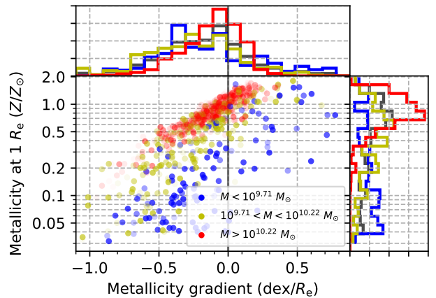
Figure 3. As Figure 2, but for mass-weighted mean metallicities and their gradients.
