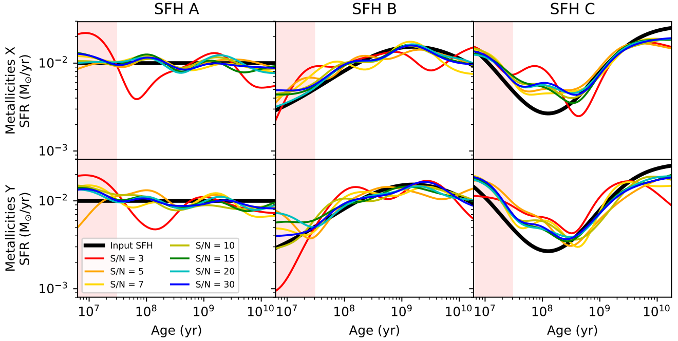
Figure A4. The measured SFHs for different input spectrum signal-to-noise ratios (coloured lines) compared to the input SFH shape (black line) for each SFH ( left to right ) and metallicity distribution ( top and bottom ). Recovered SFHs are smoothed by 0.3 dex in age. The red-shaded region indicates that for which SSP weights are ignored in science cases (see main text). The general shape is recovered well in all cases, particularly for signal-to-noise ratios greater than 5.
