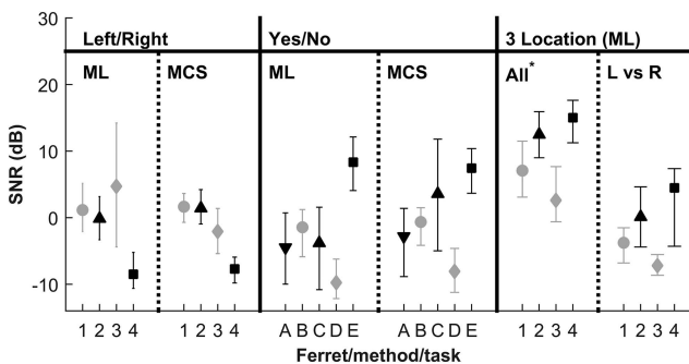
Figure 5. Comparison of individual two-location (left/right) discrimination, detection (yes/no) thresholds, signal-to-noise ratio (SNR) at 75% PC_{max} , and three-location discrimination in noise. Error bars show 95% confidence intervals. * Three-location thresholds averaged across all locations are drawn from raw % correct scores at 75%. Other data points are thresholds calculated from PC_{max} .
