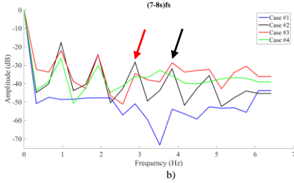
Fig. 8. FFT spectra of each S(t, f_{i,j}) for all cases for the spectral components: a) (7-6s)f_s and b) (7-8s)f_s . \Delta f = 0.4 Hz.
