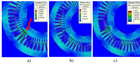
Fig. 4. a) Motors under simulation & analysis: a) Case #2, b) Case #3 and c) Case #4.
