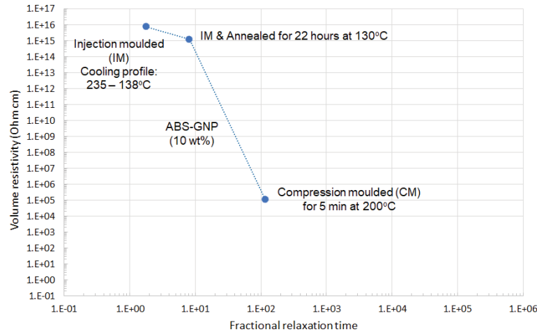
FIGURE 1. Electrical resistivity as a function of the fractional relaxation time of injection moulded, injection moulded and annealed, and compression moulded GNP-filled ABS (10 wt%). Dotted lines are a guide to the eye
